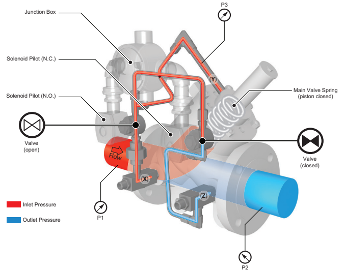
Figure 1 Closed or Closing Position
