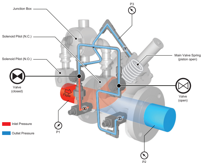
Figure 2 Full Open / No Control
