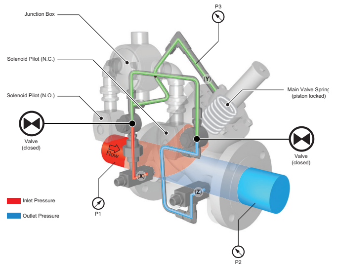
Figure 3 Controlling Position
